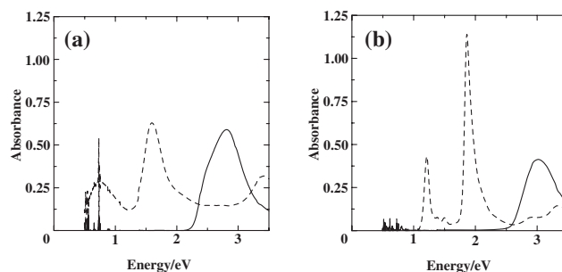
Figure 2. Electronic absorption of (a) 1 and (b) 2 : neutral (solid line) and one-electron oxidized (dashed line).
